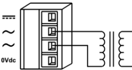
Figure 9 — AC Powered
