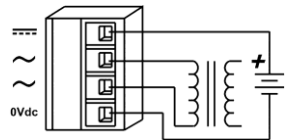
Figure 11 — AC Power with Battery Backup
