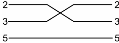
Figure 4 — Null-Modem Cable Wiring
