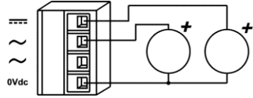
Figure 8 — Redundant DC Power
