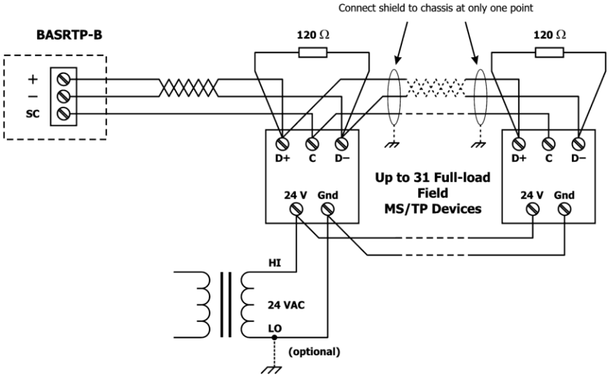
Figure 6 — 3-wire MS/TP Bus Wiring
