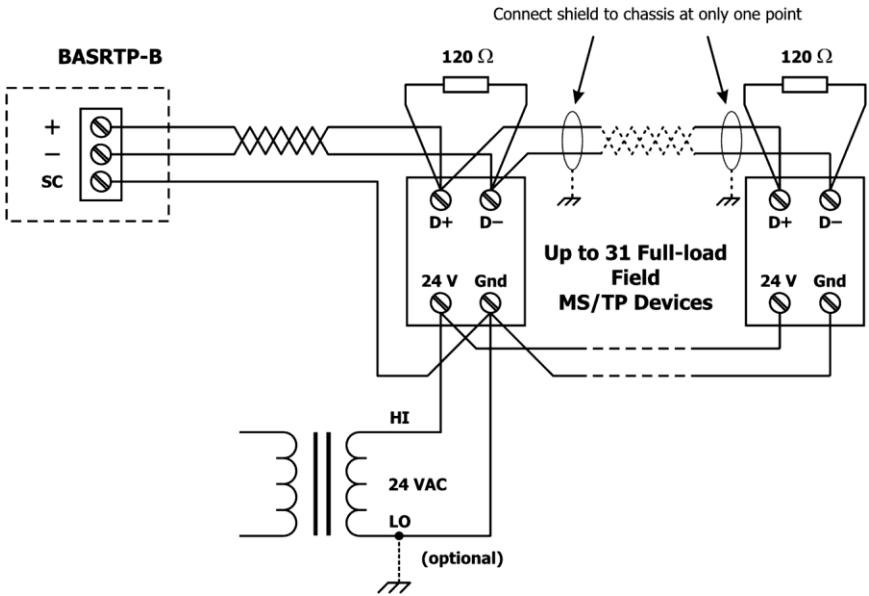
Figure 5 — 2-wire MS/TP Bus Wiring
