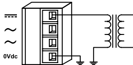
Figure 10 — AC Power with Grounded Secondary
