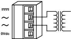
Figure 9 — AC Powered
