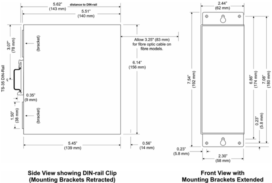
Figure 1 — EIDX Dimensions
